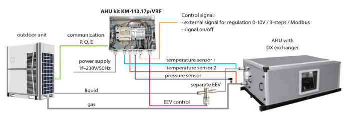
Connection scheme VRF:
