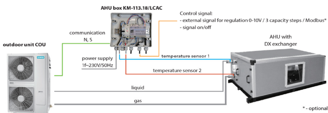
Connection scheme LCAC:
